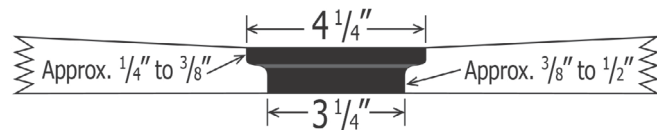
Drain Detail:
