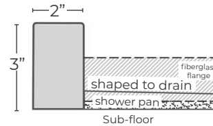
Sideview of pan w/ 1 piece curb
