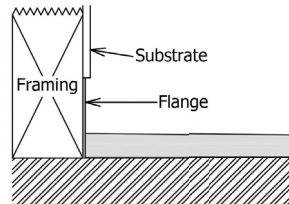
Sideview of pan w/ 1 piece curb
