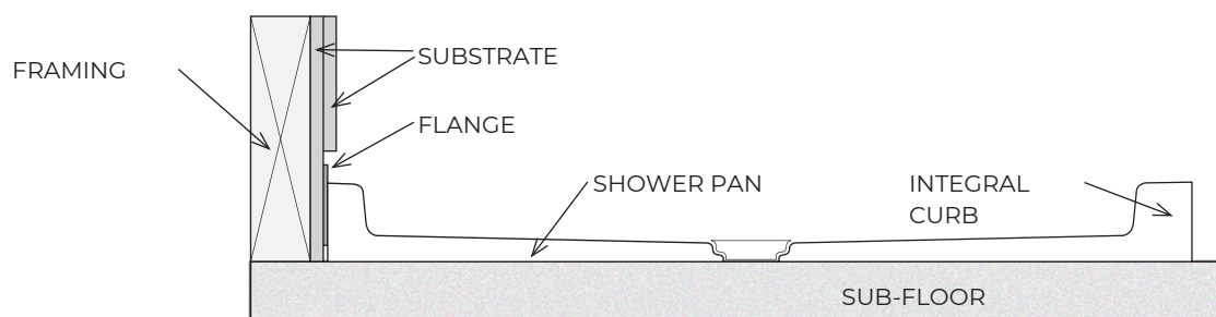
Fire-Rated Substrate Installation
